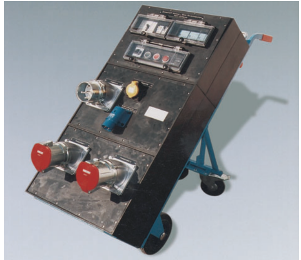
EDP-No. 43816 Pump control 55kW
