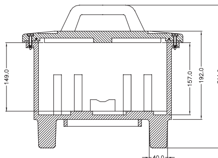
sectional view A-A (cover closed)
