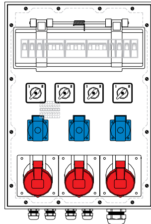
EDP-No.: 41653 Drawing-No.: 9512915
