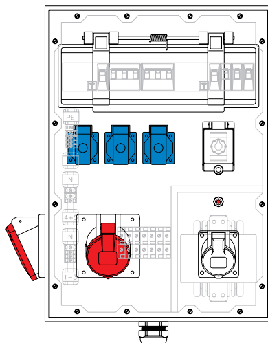
EDP-No.: 40822 Drawing-No.: 9512710
