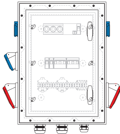
EDP-No.: 45030 Drawing-No.: 9613604
