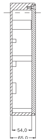
sectional view A-A
