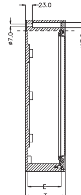
sectional view A-A
