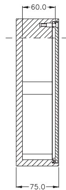
sectional view A-A
